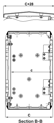
Dimensions Armoires (mm)
