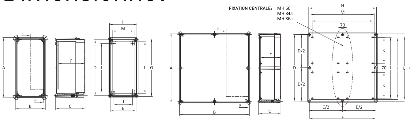
Dimensions Armoires (mm)
