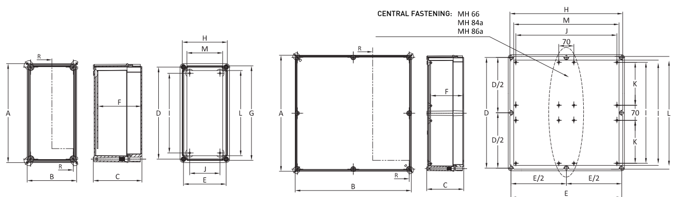
Box dimensions (mm)
