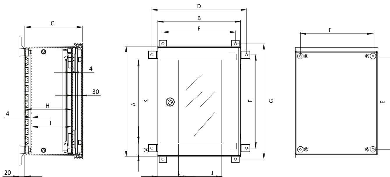
Dimensions coffrets (mm)
